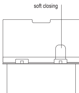
fronte / front
